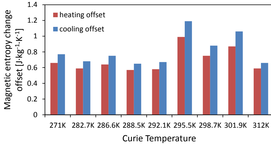
Figure 4-12 – The magnetic entropy change offset of each material for a field change from 0-1.1T.
