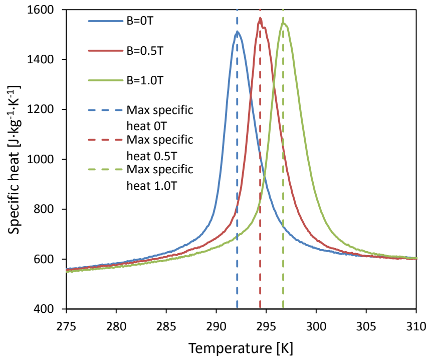
Figure 1-8 – Gadolinium ( 2^{\text{nd}} order) specific heat data [8].
