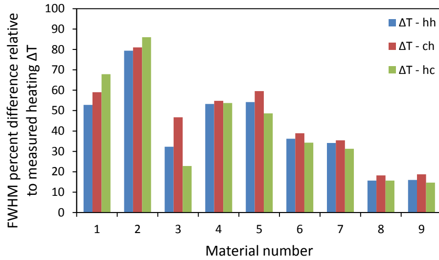
Figure 4-27 – Calculated \Delta T_{ad} FWHM relative to the measured heating \Delta T_{ad} FWHM.
