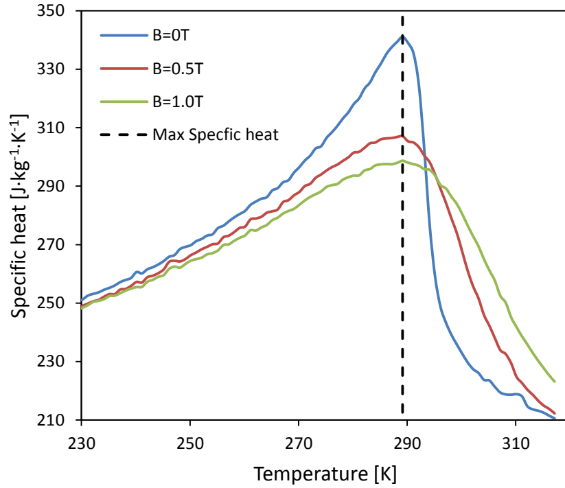
Figure 1-8 – Gadolinium ( 2^{\text{nd}} order) specific heat data [8].
