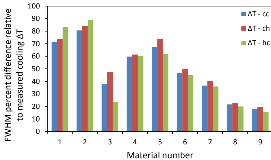
Figure 4-28 – Calculated \Delta T_{ad} FWHM relative to the measured cooling \Delta T_{ad} FWHM.
