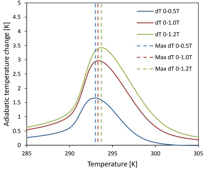
Figure 1-10 – Gadolinium \Delta T_{ad} data corrected for demagnetization [10].
