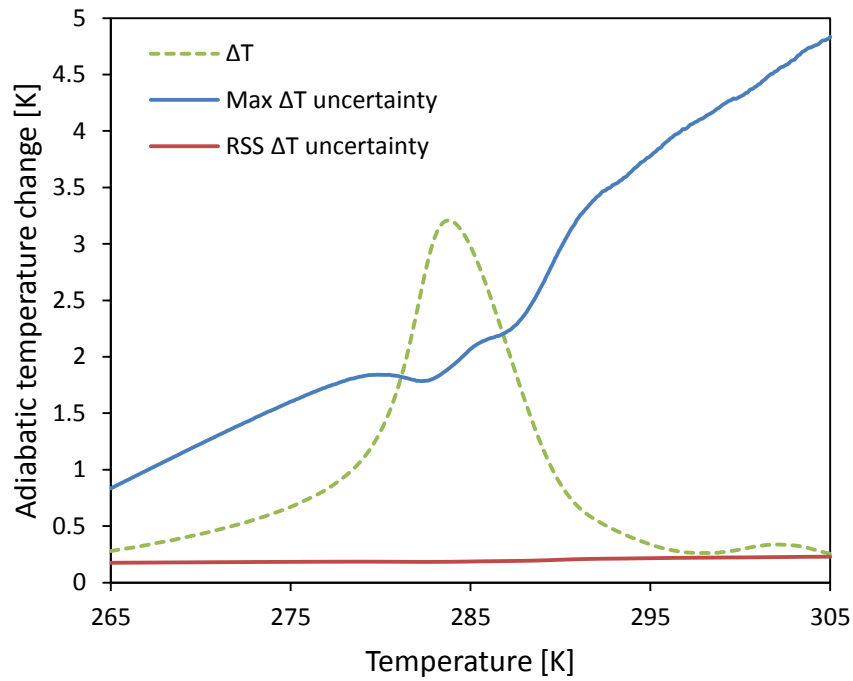
Figure 3-26 – The maximum and RSS absolute uncertainties in calculated adiabatic temperature change are plotted with the calculated adiabatic temperature change.
