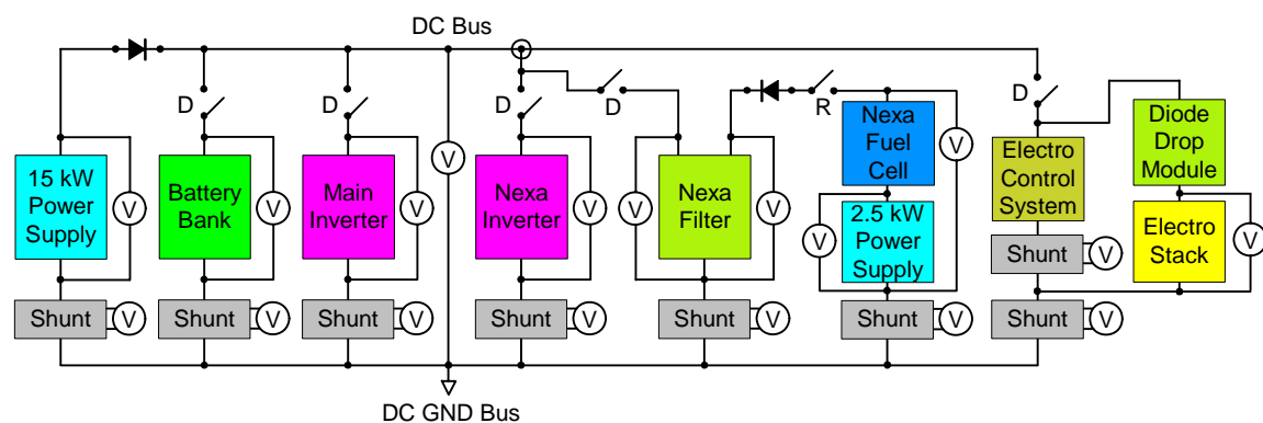
Figure 4.20 IRENE Instrumentation Node Schematic
