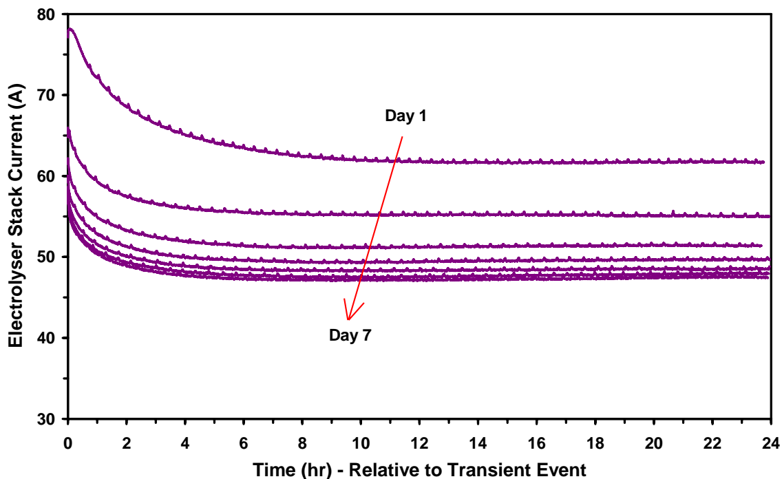
Figure 5.6 Two Minute Shutdown Response: Overlay of Daily Data from Fig. 5.5
