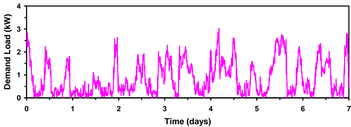
Figure 6.2 Demand Load Profile for Renewable-Regenerative Experiment
