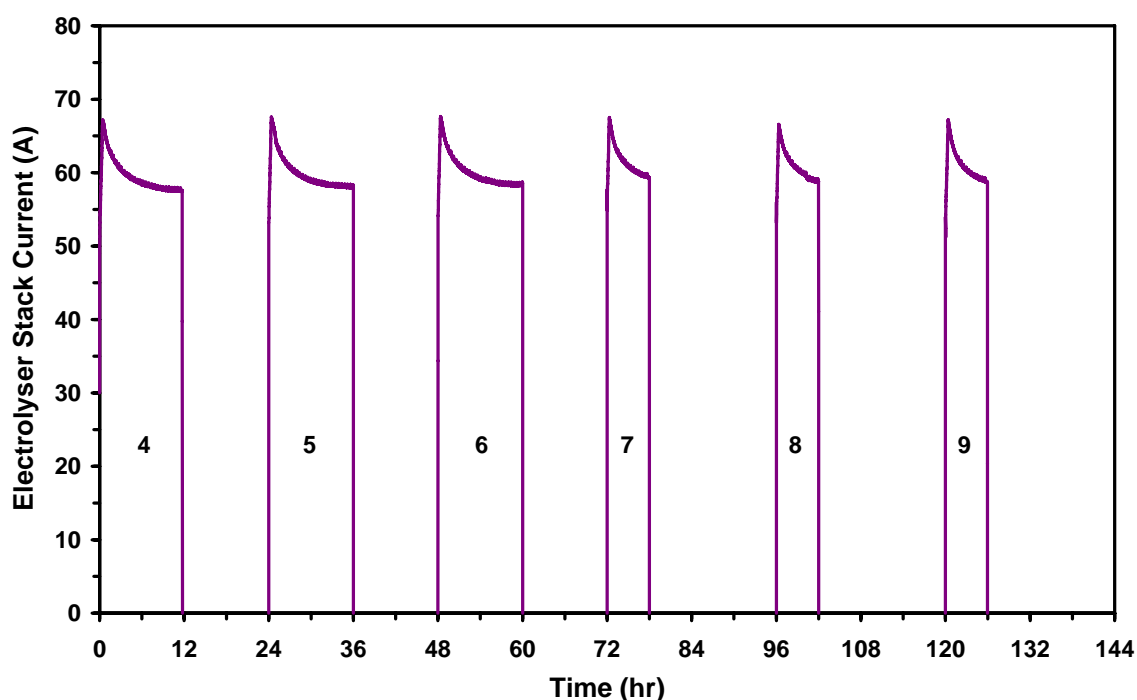
Figure 5.12 Electrolyser Response to 24 Hour Operating Cycles
