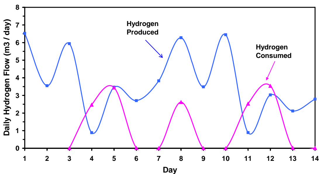
Figure 6.6 Daily Hydrogen Production and Consumption
