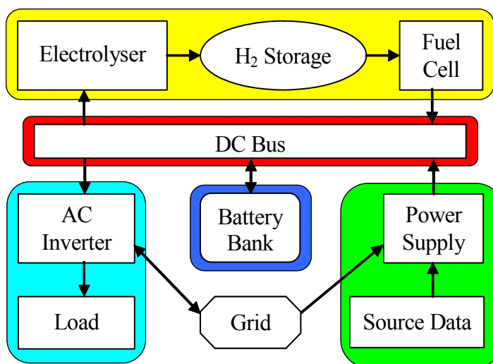
Figure 3.1 IRENE Test Platform Schematic
