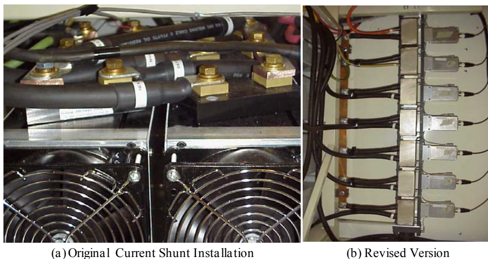
Figure 4.21 DC Bus Current Measurement Configuration
