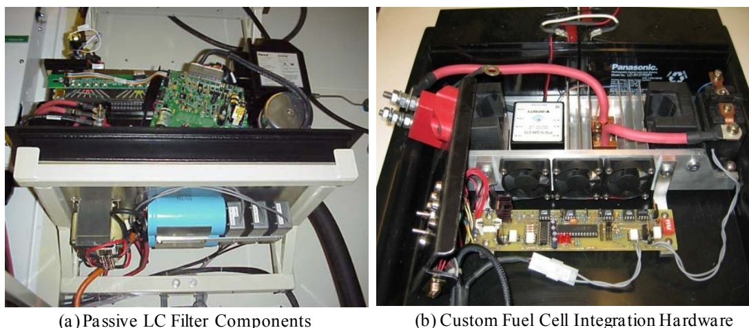
Figure 4.19 Nexa Integration Components
