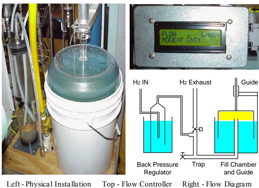
Figure 4.10 Inverted Bucket Flow Meter
