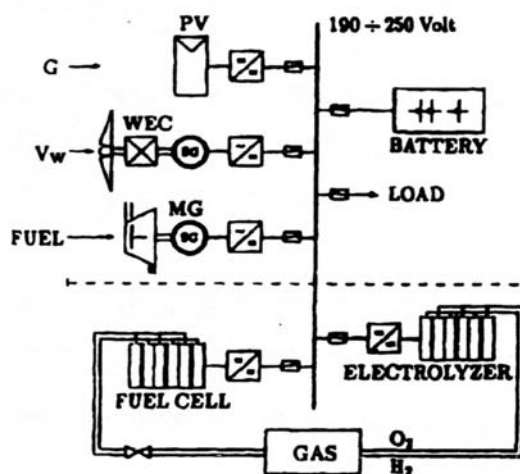
Figure 2.6 University of Oldenburg Renewable Energy Test Facility
