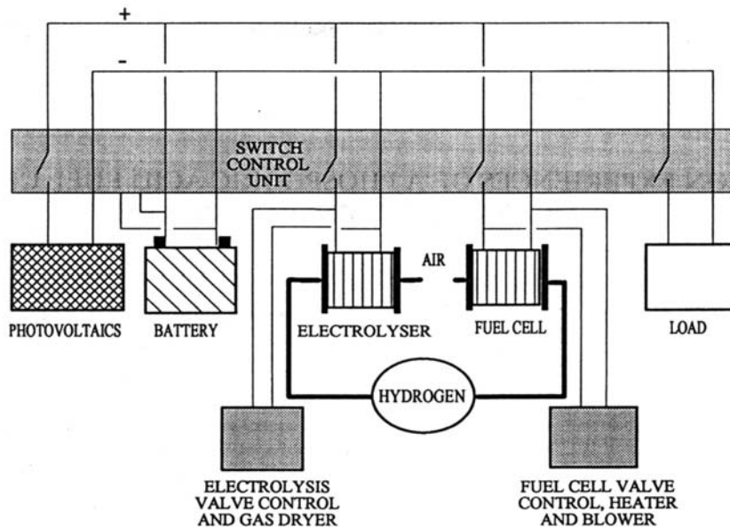
Figure 2.3 University of Helsinki Hydrogen Energy Test Facility Schematic
