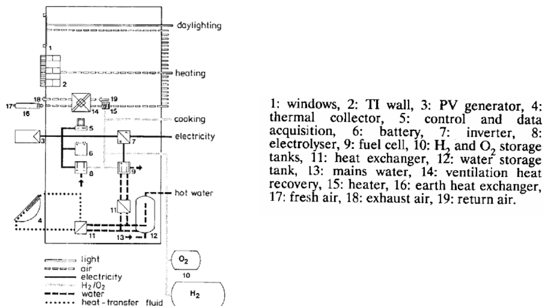
Figure 2.5 Freiburg Self-Sufficient Solar House Energy System Diagram
