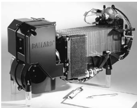
Figure 3.8 Nexa Fuel Cell
