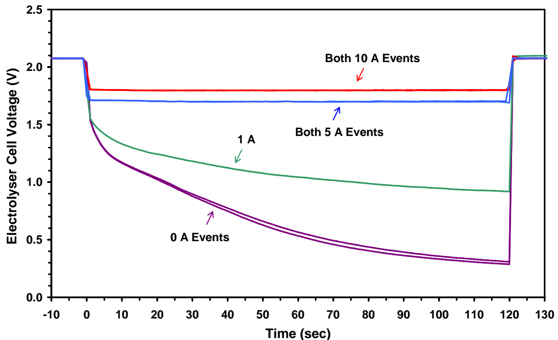
Figure 5.9 Electrolyser Stack Voltage During Two Minute Transition Events
