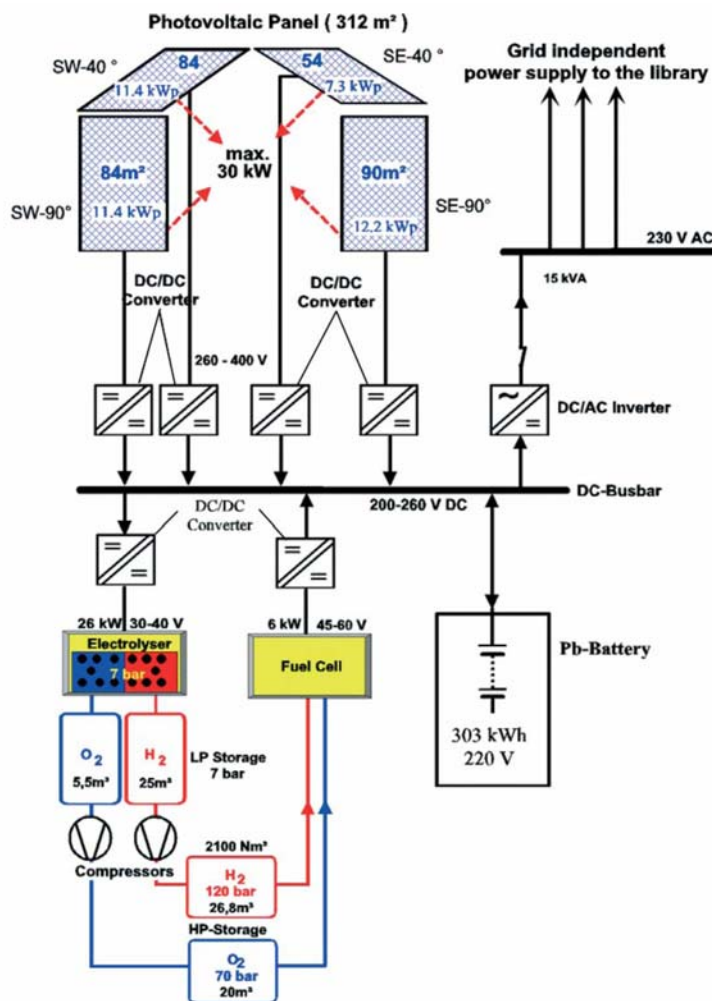
Figure 2.10 PHEOBUS Block Diagram
