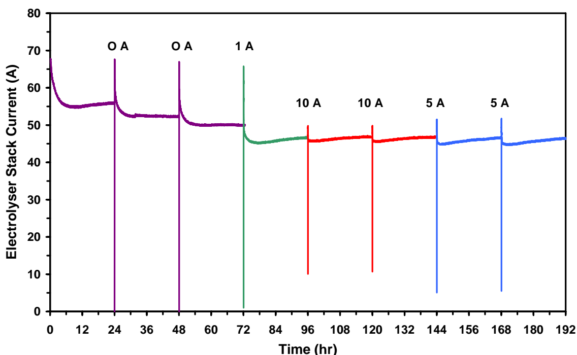
Figure 5.7 Electrolyser Response to Minimum Holding Current
