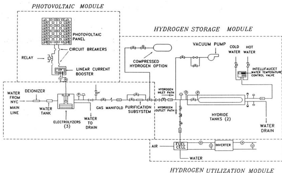
Figure 2.9 The Copper Union Hydrogen Energy Test Facility Schematic
