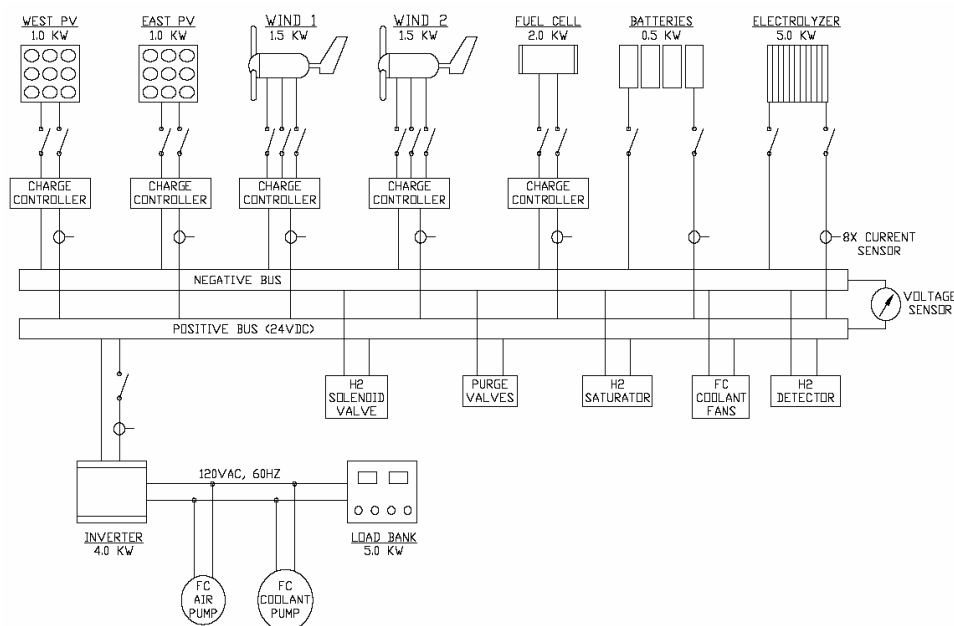
Figure 2.14 Desert Research Institute Hybrid Hydrogen Energy Facility Schematic
