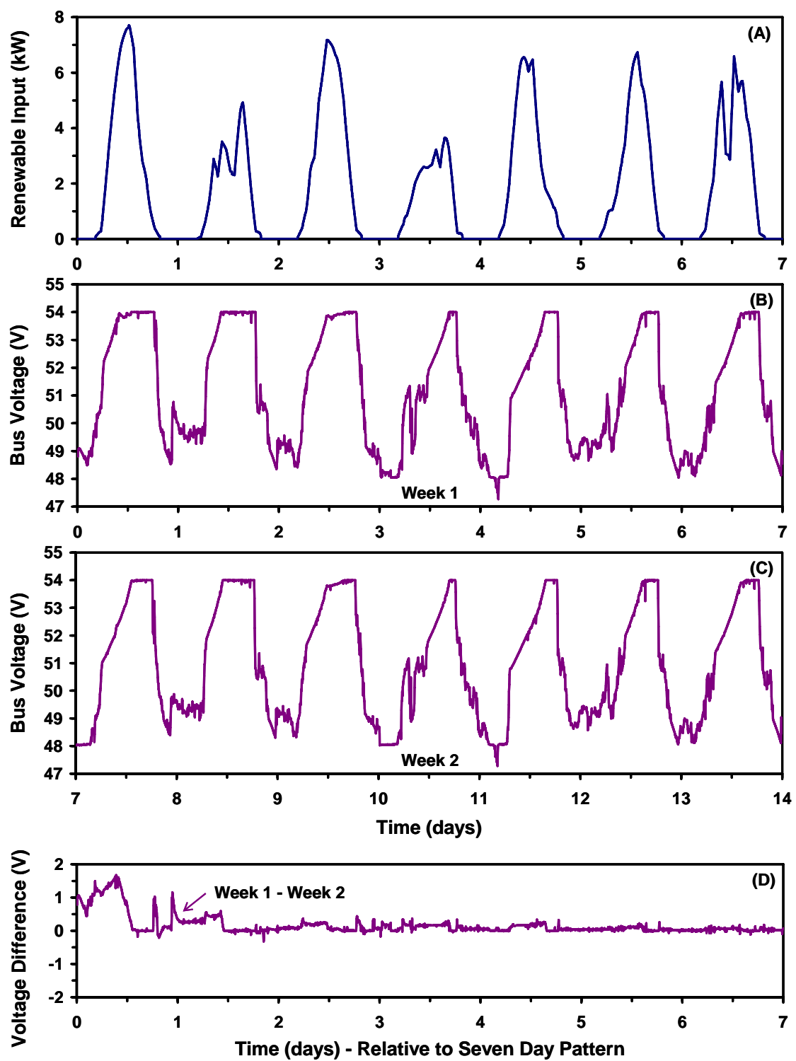
Figure 6.9 Bus Voltage Dynamics
