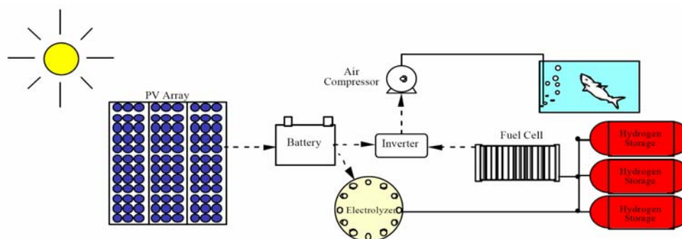
Figure 2.4 Schatz Solar Hydrogen Project Schematic
