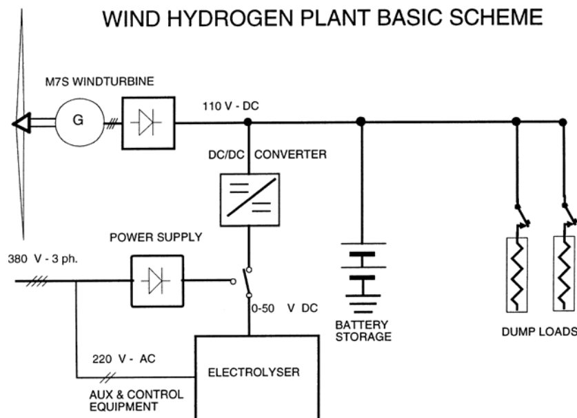
Figure 2.11 ENEA Wind Hydrogen Plant Schematic
