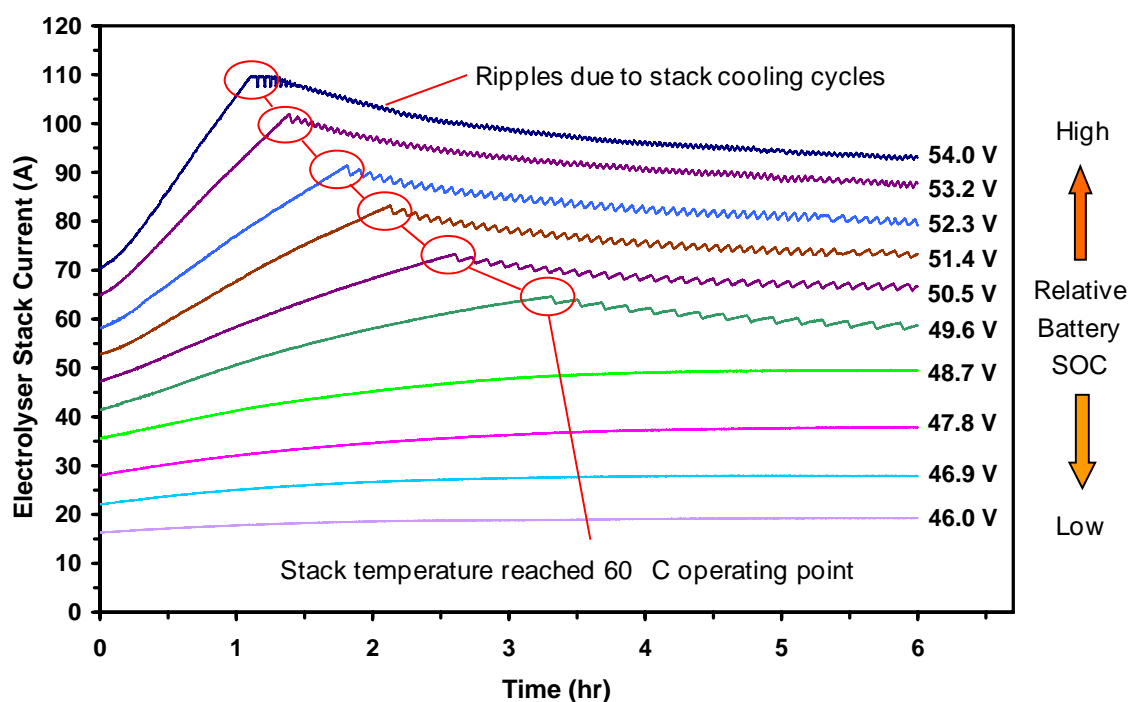
Figure 5.2 Electrolyser Six Hour Step Function Response
