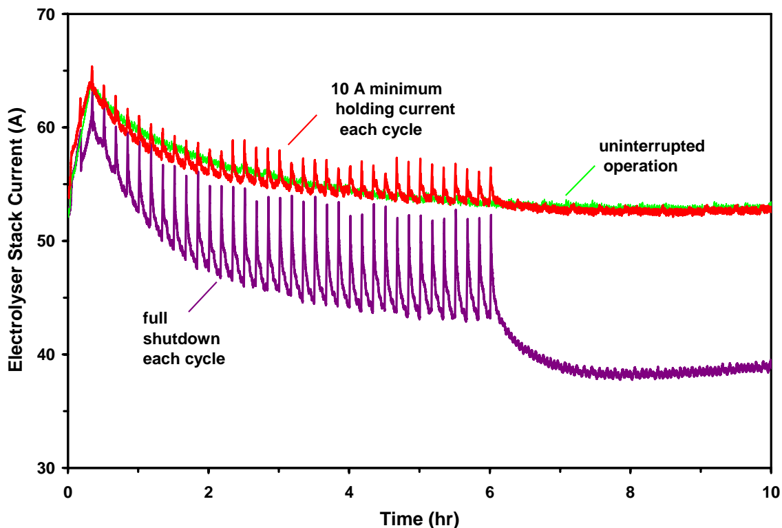
Figure 5.10 Electrolyser Response to Rapid Cycling
