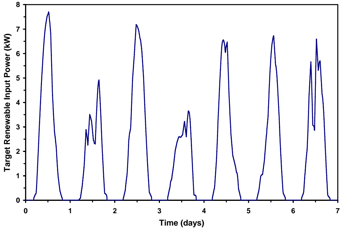
Figure 6.1 Resource Input Power Profile for Renewable-Regenerative Experiment
