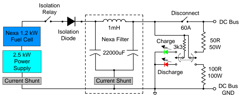
Figure 4.18 Nexa Integration Schematic
