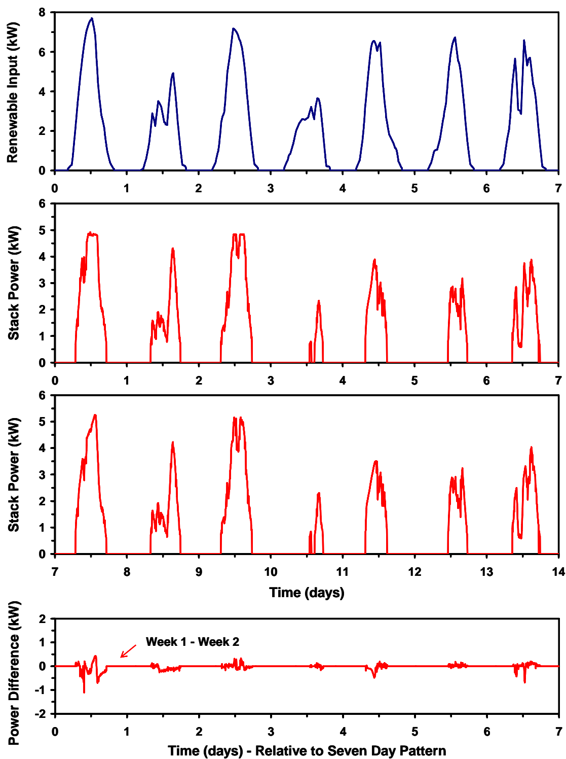
Figure 6.12 Electrolyzer Input Power Profile
