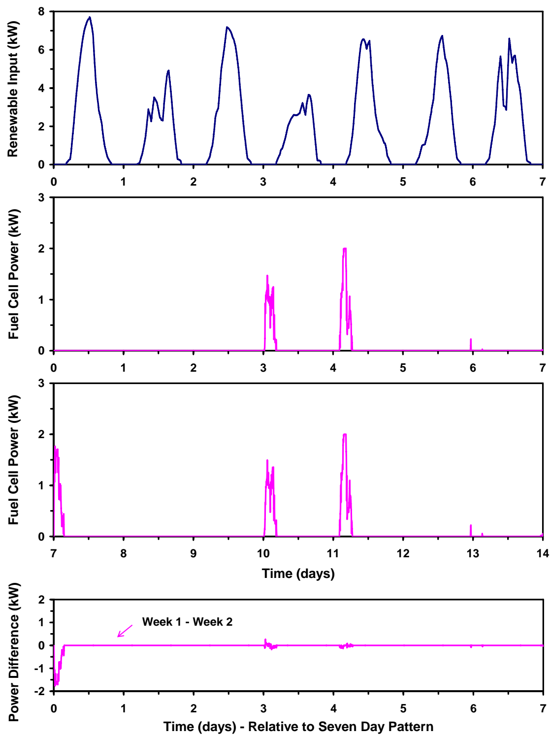
Figure 6.10 Fuel Cell Power Contribution
