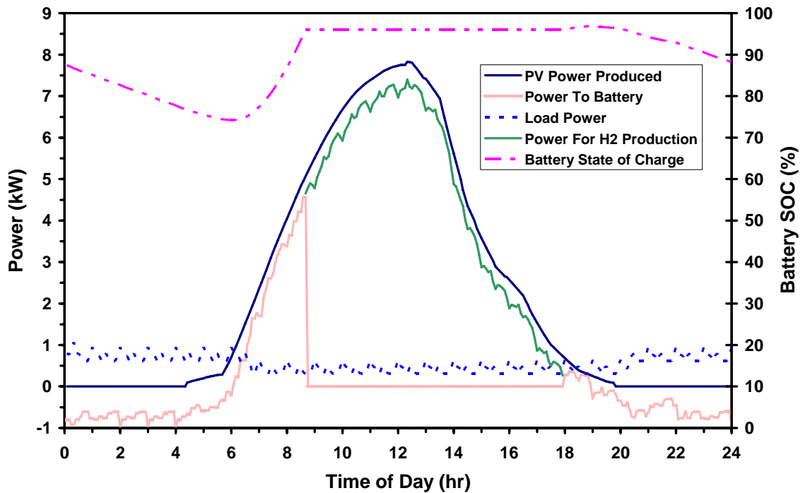
Figure 5.1 Input Power Profile Reference Data – NRCan Model
