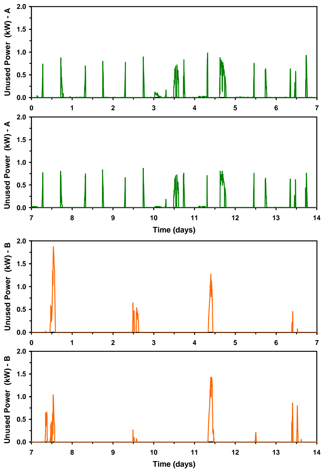
Figure 6.13 Unused Renewable Input: A) Electrolyser Threshold, B) Transition Rate
