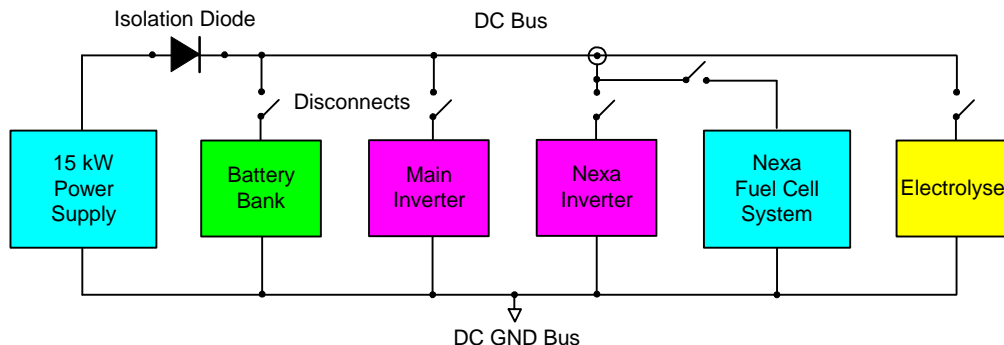
Figure 4.2 Simplified DC Bus Schematic
