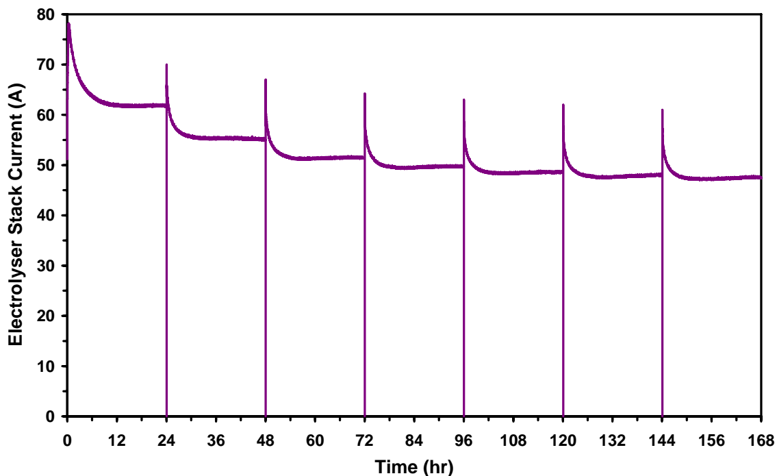
Figure 5.5 Electrolyser Response to Repeated Two Minute Shutdowns
