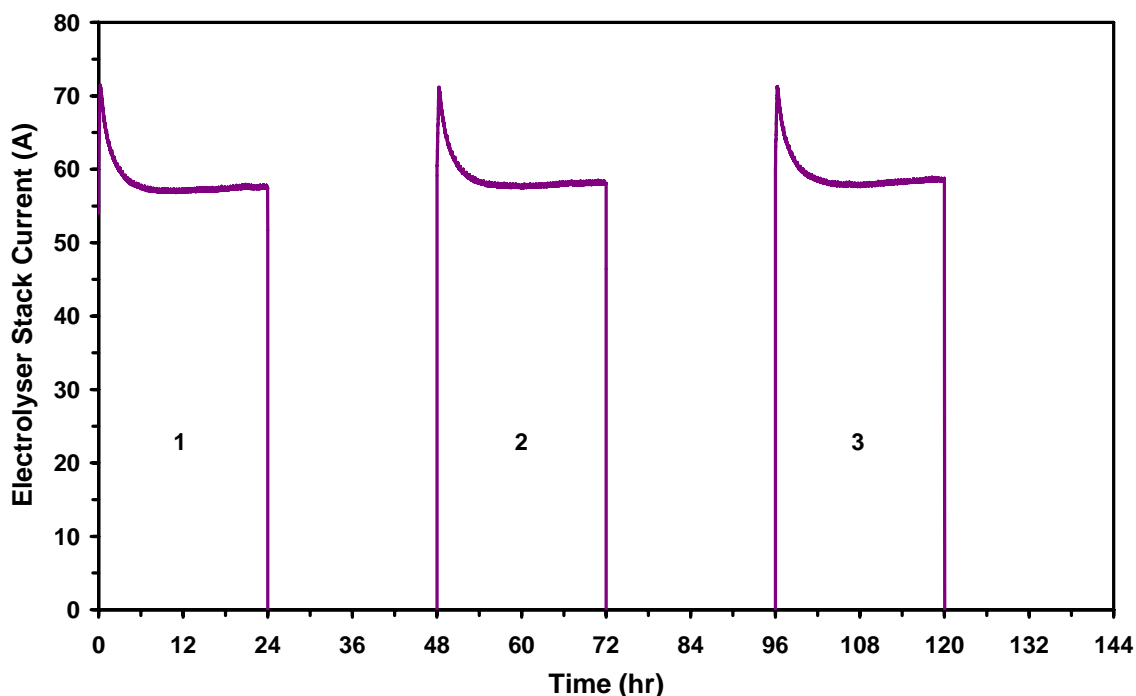
Figure 5.11 Electrolyser Baseline Response to 48 Hour Operating Cycle
