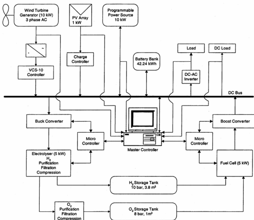
Figure 2.13 Hydrogen Research Institute Test Facility Block Diagram
