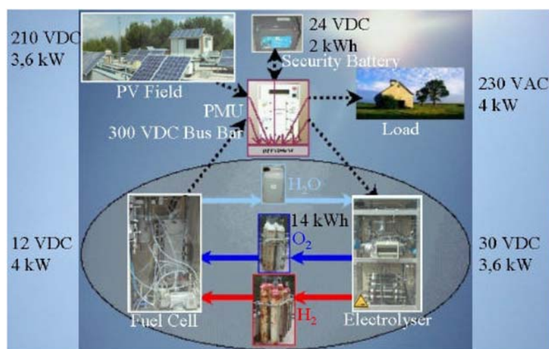
Figure 2.16 PVFC Hydrogen Energy System Conceptual Diagram
