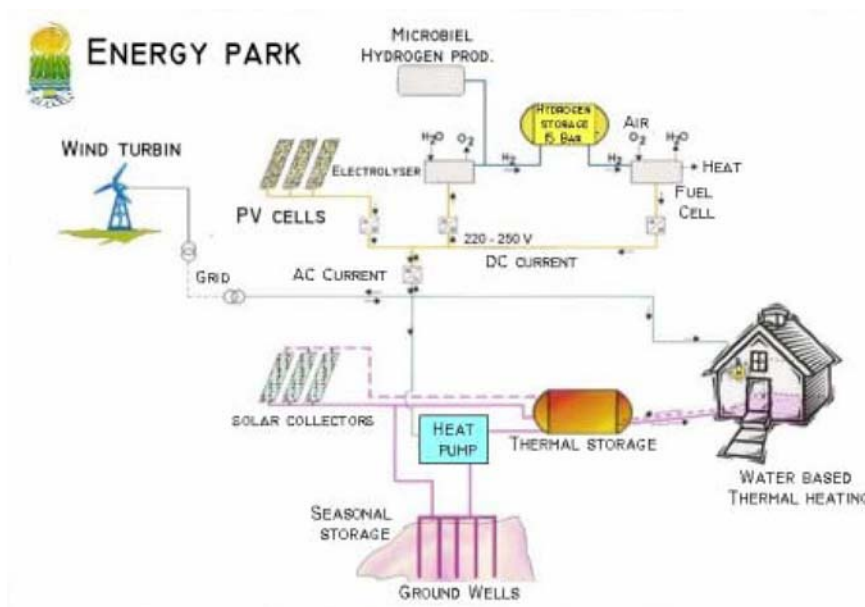
Figure 2.15 Renewable Energy Park Component Diagram
