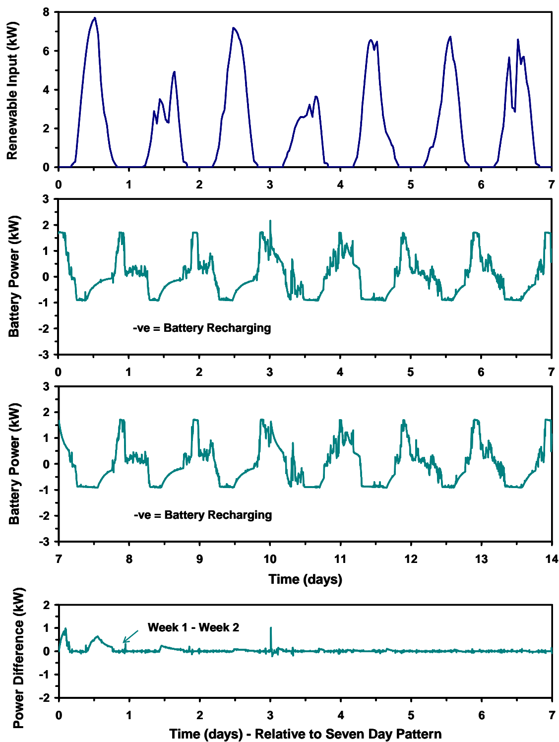
Figure 6.11 Battery Power Delivered to IRENE System
