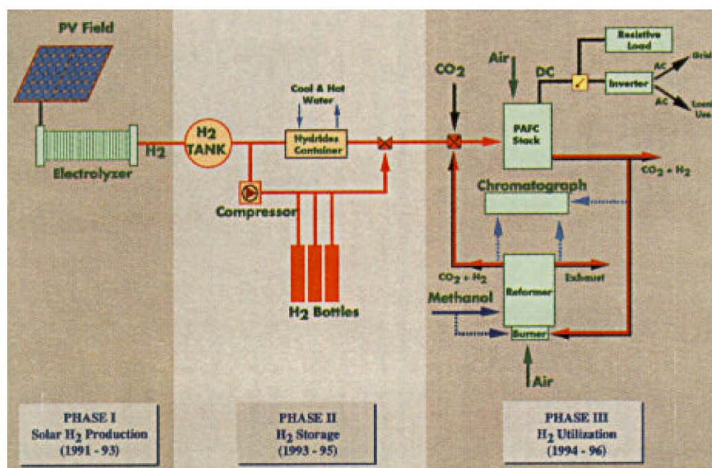
Figure 2.7 INTA Solar Hydrogen Energy Test Facility Block Diagram
