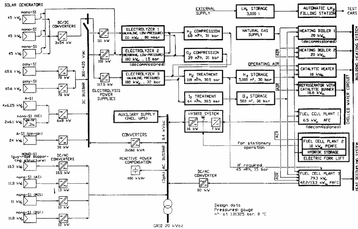
Figure 2.2 SWB Solar Hydrogen Facility Block Diagram
