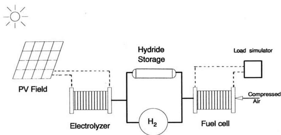
Figure 2.12 SYMPHYS Schematic Diagram
