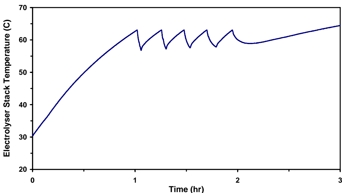
Figure 4.11 Electrolyser Stack Temperature Response at 100 A Input Current
