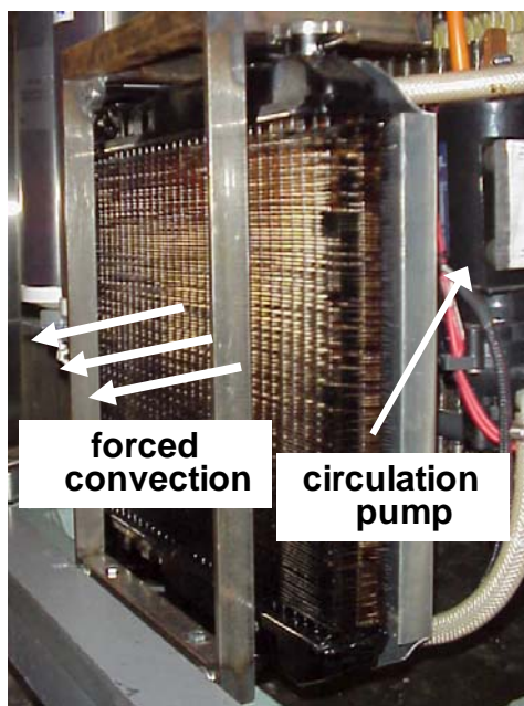
Figure 4.12 Electrolyser Cooling System Upgrades
