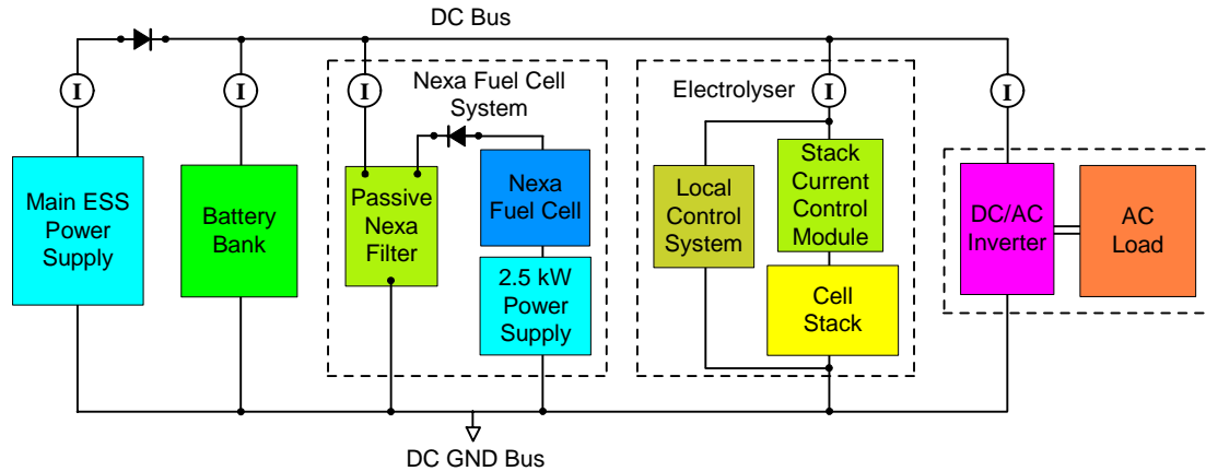
Figure 6.4 IRENE Hardware Configuration Schematic
