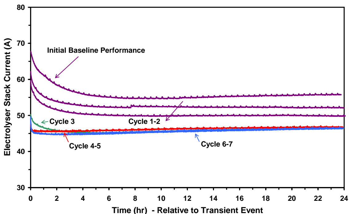
Figure 5.8 Hold Current Response: Overlay of Daily Data from Fig. 5.7
