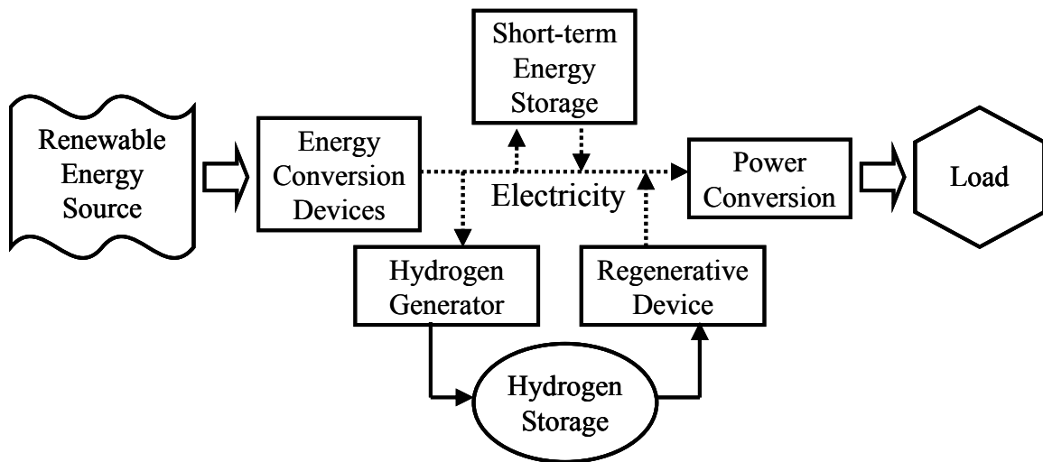
Figure 2.1 Typical First Generation Renewable-Regenerative System Architecture
