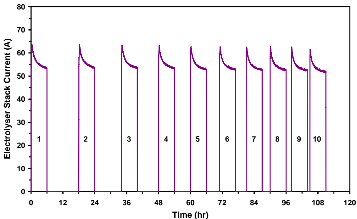
Figure 5.13 Electrolyser Response to Variable Duration Rest Periods
