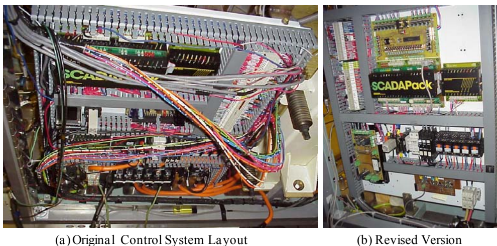
Figure 4.13 Electrolyser Instrumentation a Control System Upgrades
