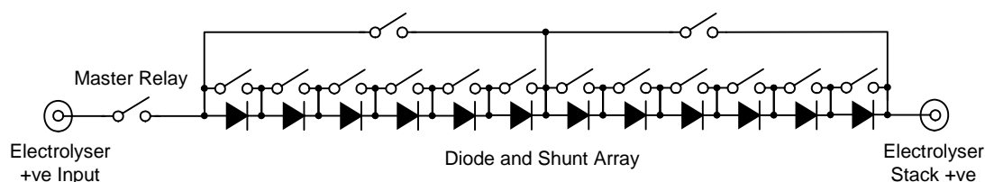
Figure 4.14 Electrolyser Diode Power Conditioner Schematic
