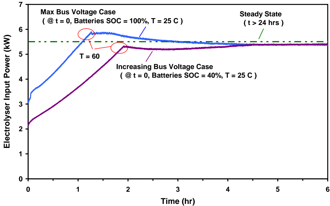
Figure 5.3 Coupled Electrolyser Operation and Battery Charging
