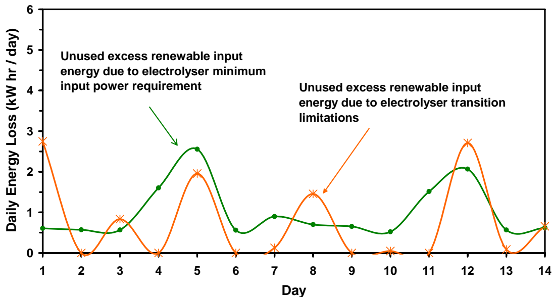
Figure 6.8 Daily Breakdown of Electrolyser Energy Losses
