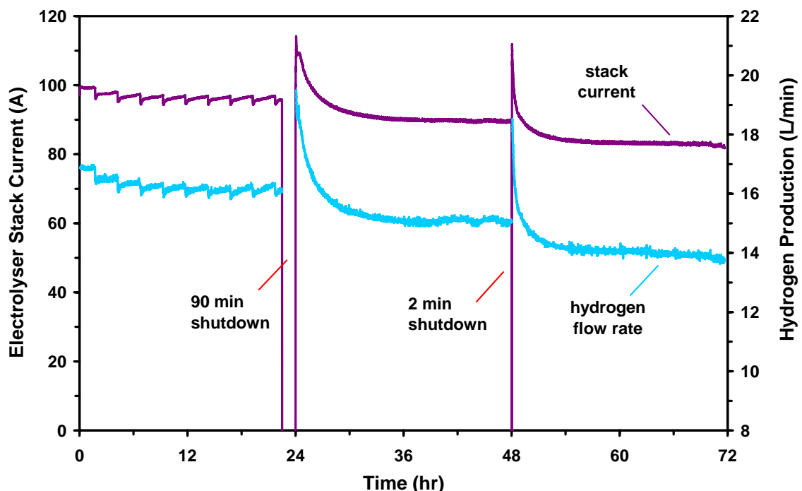
Figure 5.4 First Observation of Dynamic Induced Electrolyser Performance Decline
