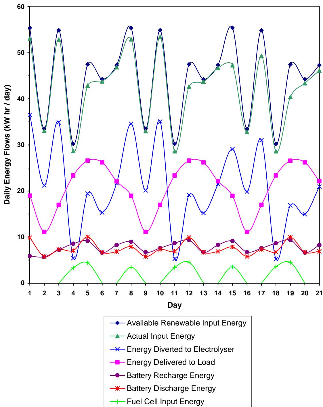
Figure 6.5 Daily Energy Balance for Three Week IRENE System Experiment
