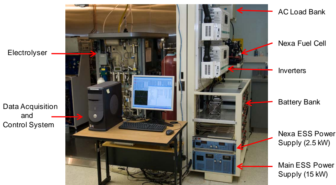
Figure 4.1 IRENE System Installation
