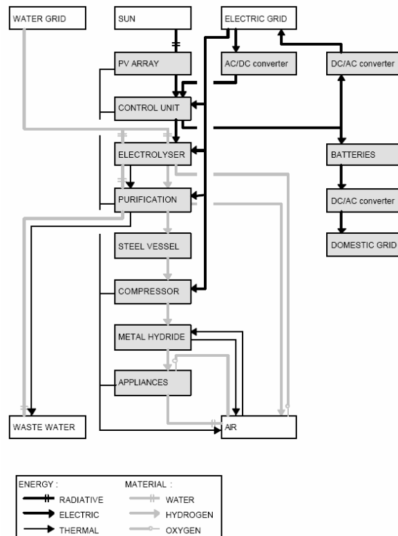
Figure 2.8 Friedli Residential Solar Hydrogen House Energy System Block Diagram
