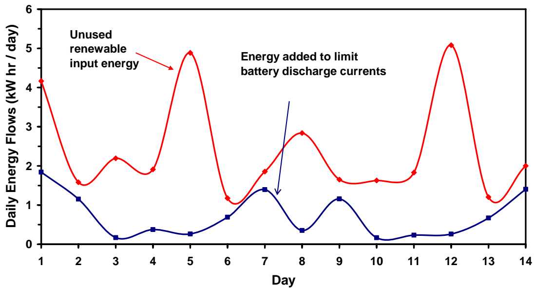
Figure 6.7 Daily Energy Supplement and Losses
