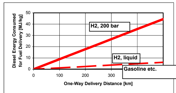
Figure 6 Road delivery of hydrogen
