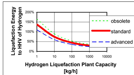
Figure 5 Liquefaction of hydrogen gas
