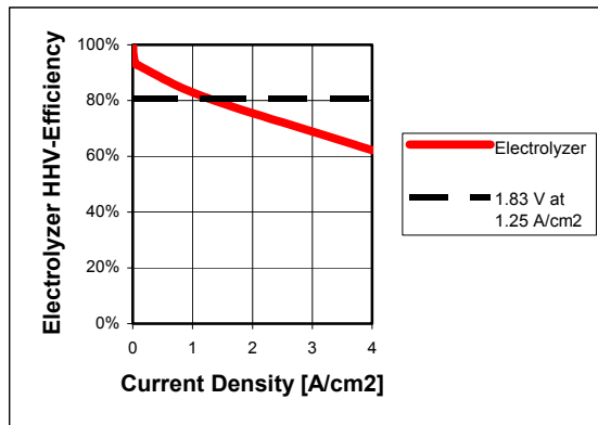
Figure 3 Energy losses of hydrogen production by electrolysis.
