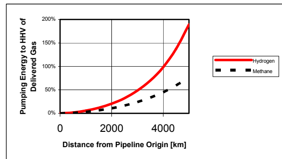
Figure 7 Long distance transport of hydrogen through pipelines
