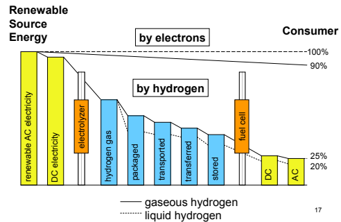
Figure 9 Transport of renewable electricity by electrons and by hydrogen. Only about 25% of the original energy becomes useful for the hydrogen path
