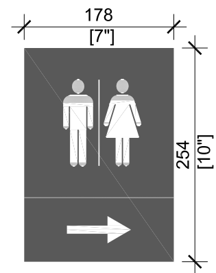
To Separate Men's and Women's Washrooms [WID6a]
