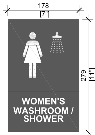
Women's Washroom / Shower [WID13]
