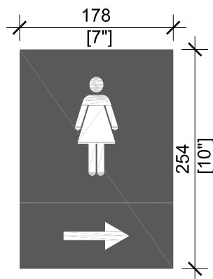
To Women's Washroom [WID4a]
