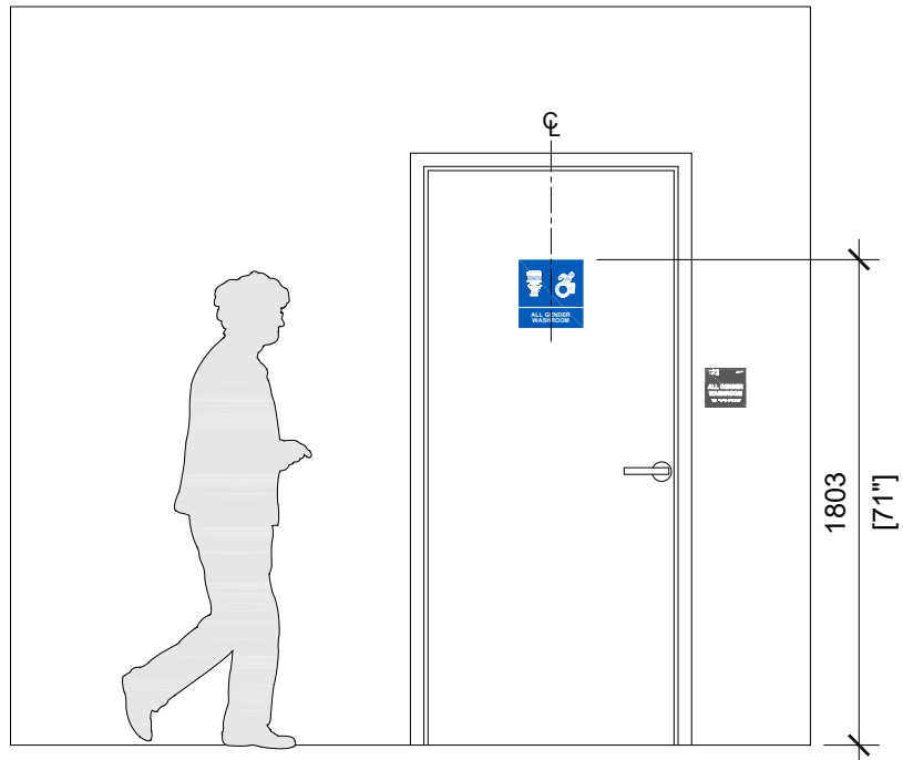
Installation of Washroom Door Signs
