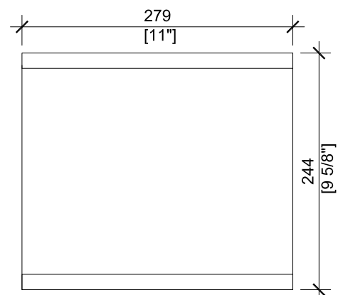
Wall Mounted Sign Holder [N3d] with Landscape Letter Size opening
