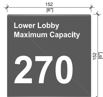
Unenclosed Room Occupant Load Sign [ID7a]
