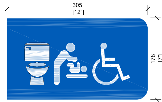
Accessible All Gender Washroom w/ Change Table [WP22]
