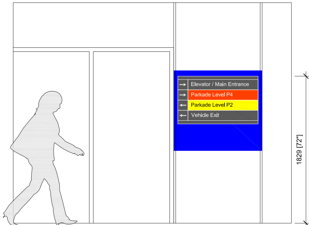
Typical Installation of Large Wall Mounted Wayfinding [W1b] on flush surface
