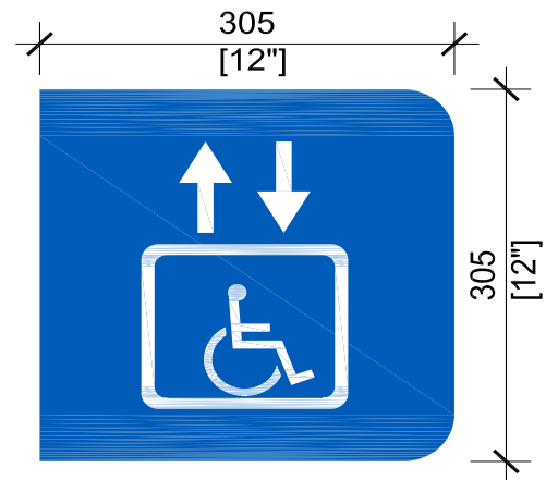
Projecting Accessible Elevator Sign [P6 / P6-45]
