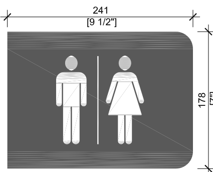
Separate Men's and Women's Washrooms [WP6-45]
