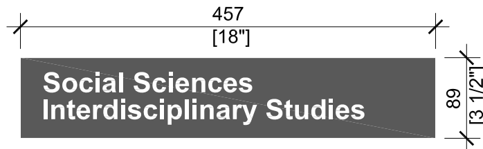
Projecting Office Information Sign [PID1b]
