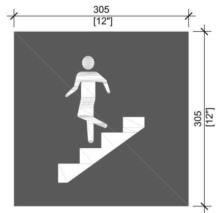
Stairwell Graphic Sign [S4]
