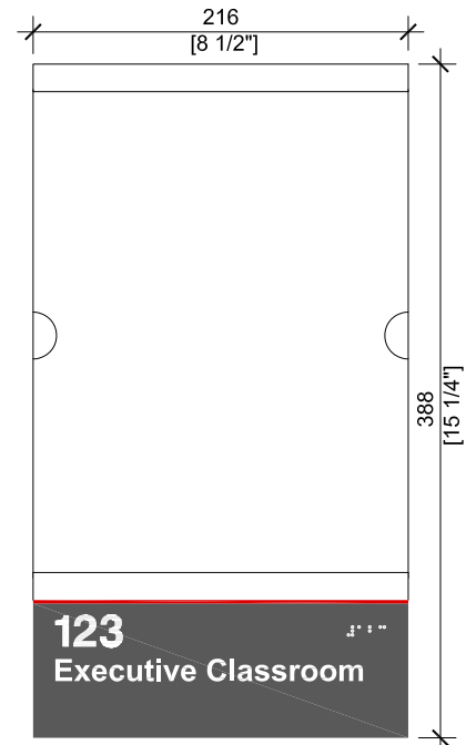
Single-Line Wall-Mounted Room Number Sleeve [ID9a] with engraved text
