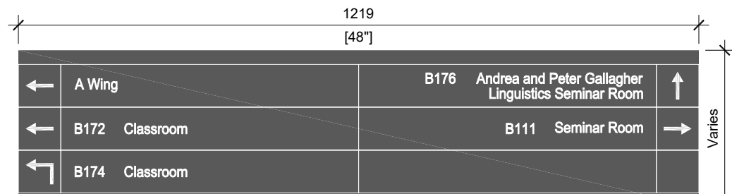
Double-Wide Wall Mounted Wayfinding [W1a]
