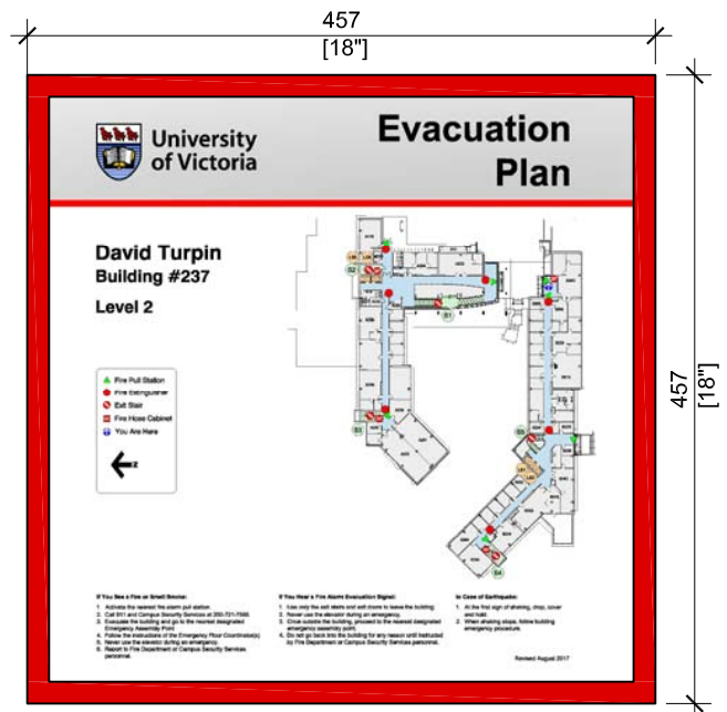
Evacuation Plan Sign [E1 / E2]
