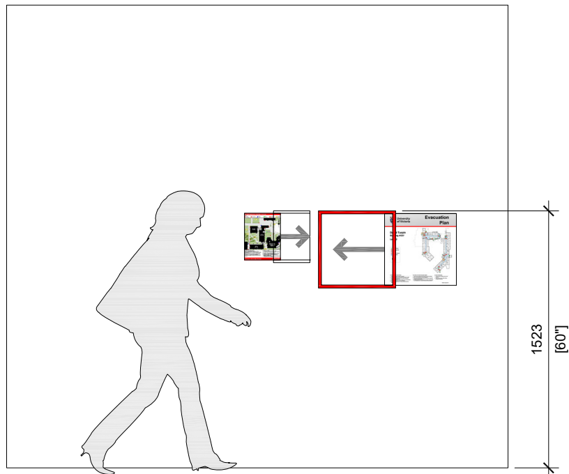
Installation of Evacuation Plan [E1 / E2]. E1 shown beside N6d with insert being inserted into right side.
