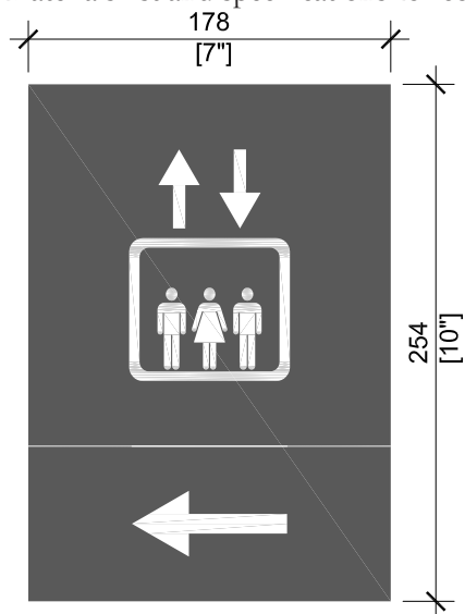
Elevator Directional Sign [SE1]
