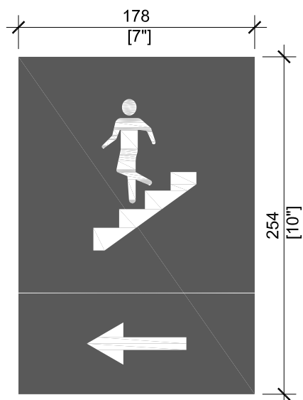
Stairwell Directional Sign [SE2]
