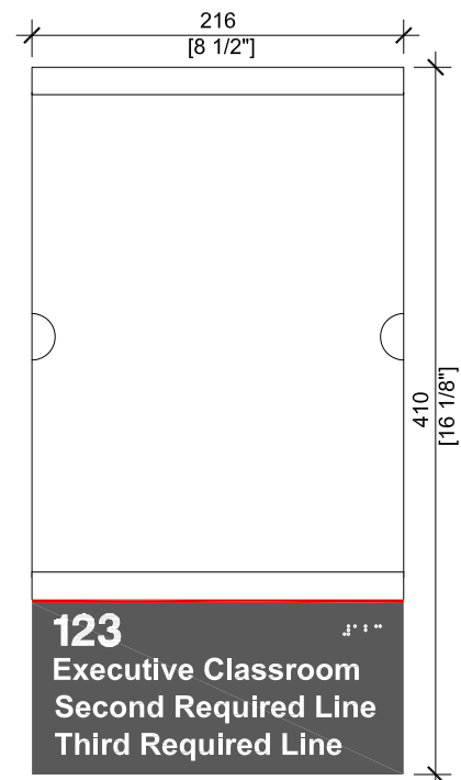
Multiple-Line Wall-Mounted Room Number Sleeve [ID9b] with engraved text
