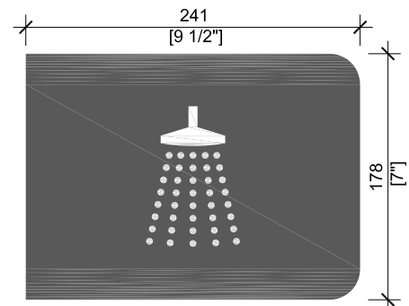
45 Degree All Gender Shower [WP21-45]
