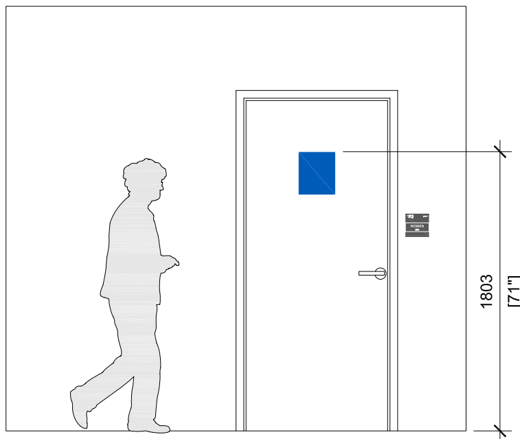
Installation of Washroom Backing Sign shown to accommodate WID15 & WID16 Signs
