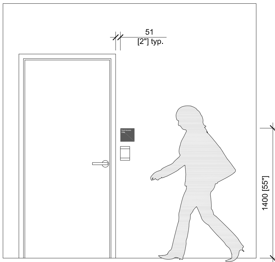
Installation of Door Information Plate [ID12]
