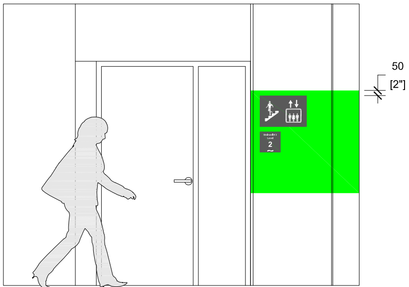
Installation of Stairwell / Elevator Graphic Sign [S3], shown above S1
