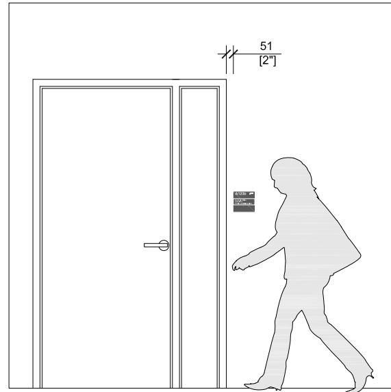
An installation beside sidelight measuring less than 305mm wide
