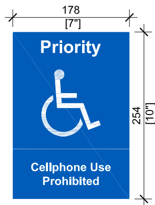
Accessible Priority Use [WS1]
