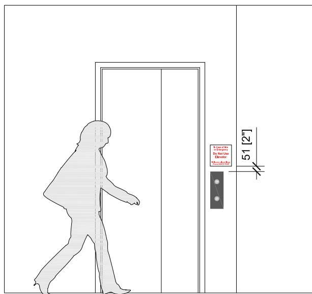
Alternative Installation of Elevator In Case of Emergency Sign [S8]
