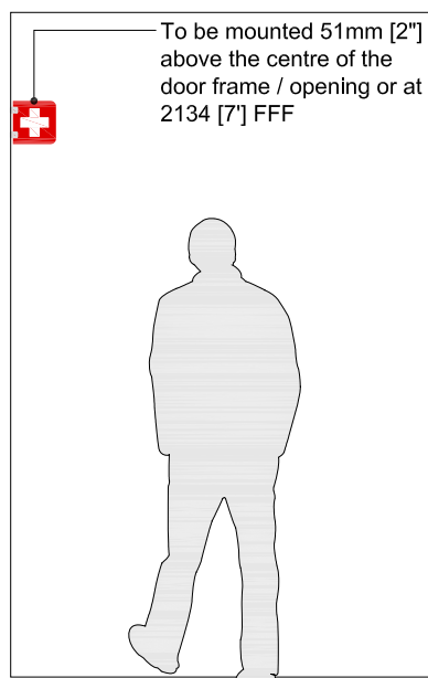
Installation of Projecting First Aid Sign [PID10]
