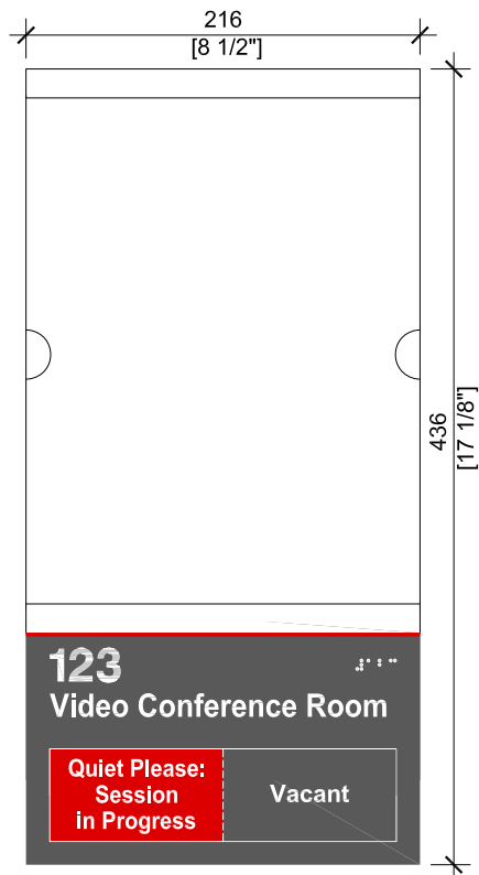
Wall-Mounted Meeting Room Sleeve with Red Warning Plate [ID8c]
