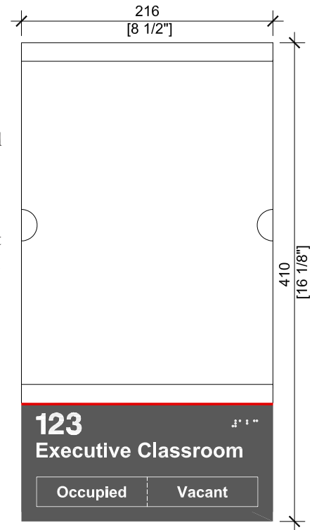
Wall-Mounted Meeting Room Sleeve [ID8a]
